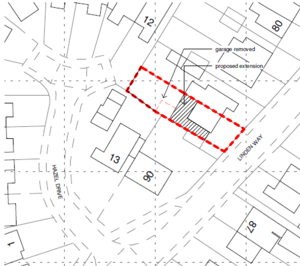
Block Plan
