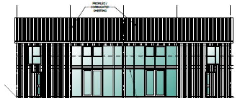
PROPOSED SOUTH EASTERN ELEVATION
