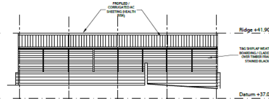
EXISTING SOUTH WESTERN ELEVATION
