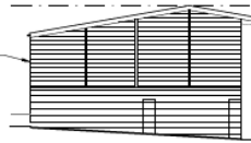
PROPOSED SOUTH EASTERN ELEVATION
